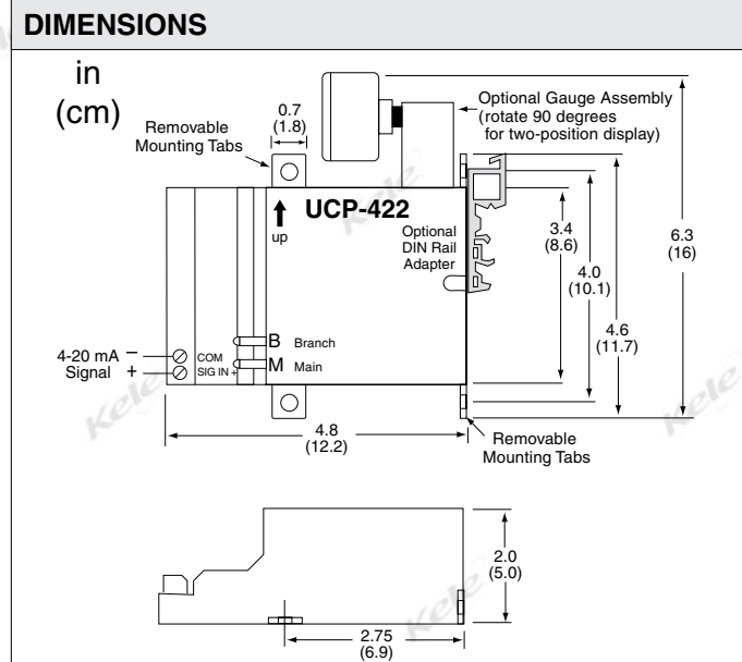
UCP-422-43 (Shown with Optional Pressure Gauge)
